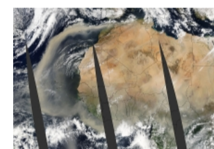
A 'green' Sahara was far less dusty than today
