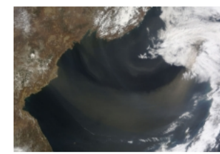
Intensity of desert storms may affect ocean phytoplankton
